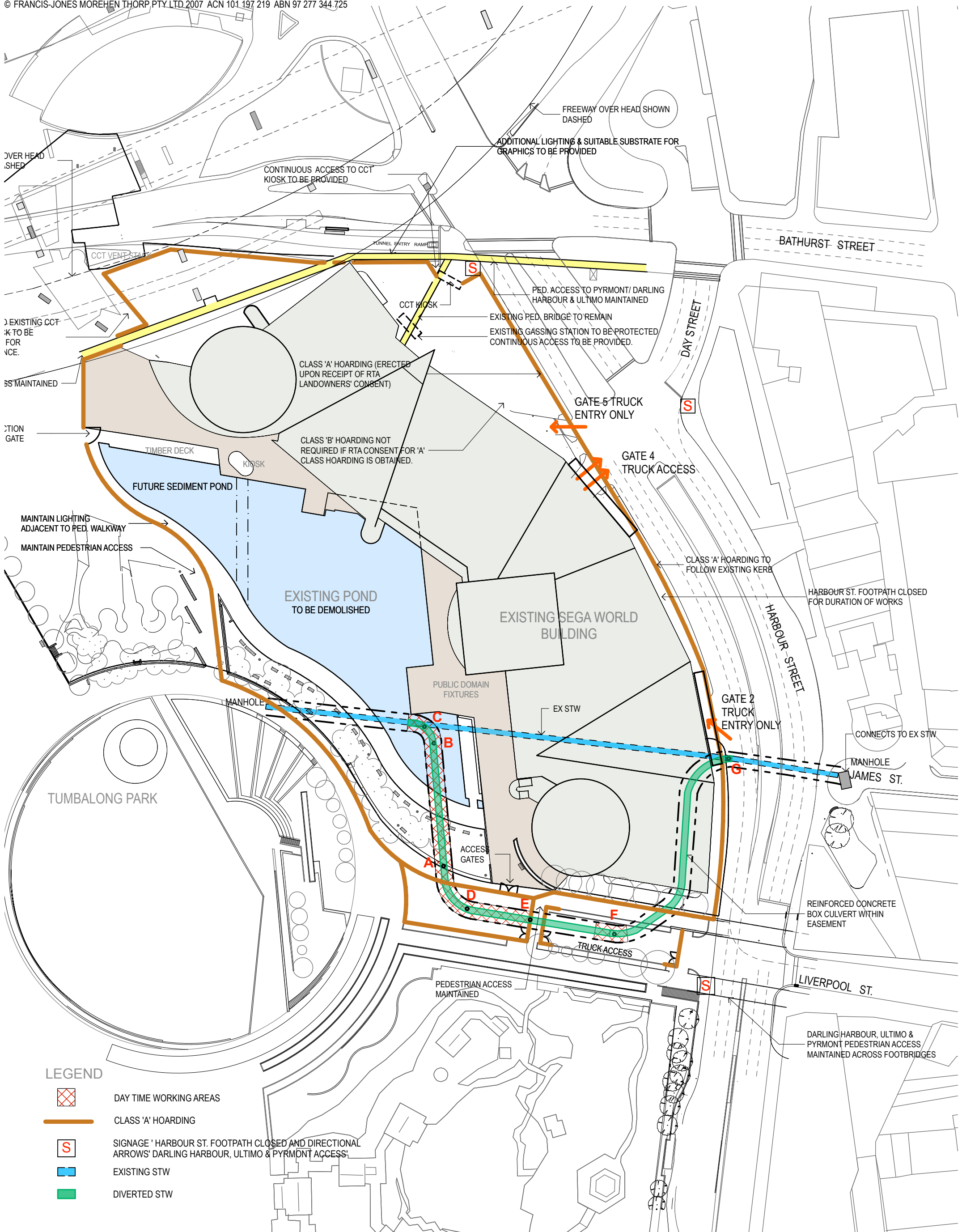
STORMWATER DIVERSION & HOARDINGS CONCEPT PLAN - STAGE 01 1:1000
